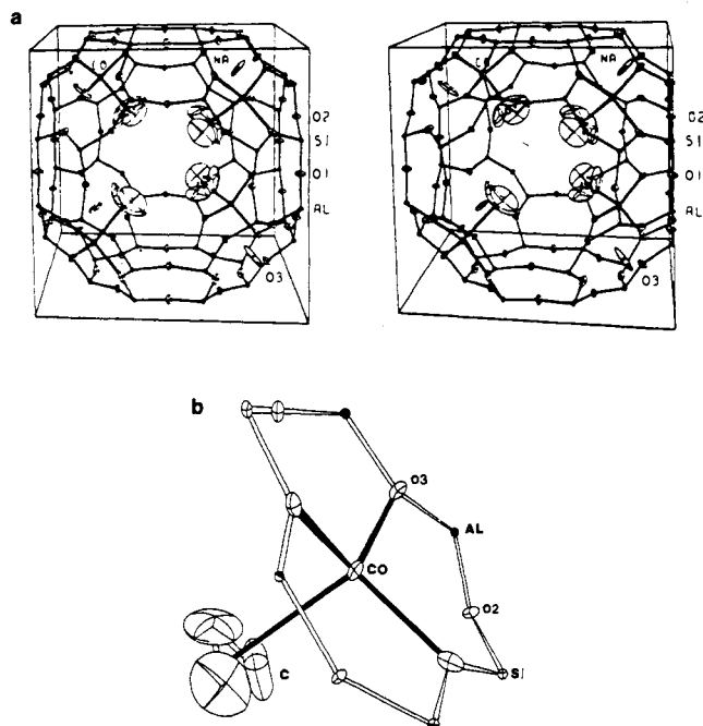
Figure 10. Intrazeolite cyclopropane complex of Co(II) in zeolite A. (a) Stereoview of the Co 4 Na 4 A·4C 3 H 6 unit cell. (b) Coordination environment of the Co(II) ion. Reprinted from ref 45; copyright 1978 American Chemical Society.
