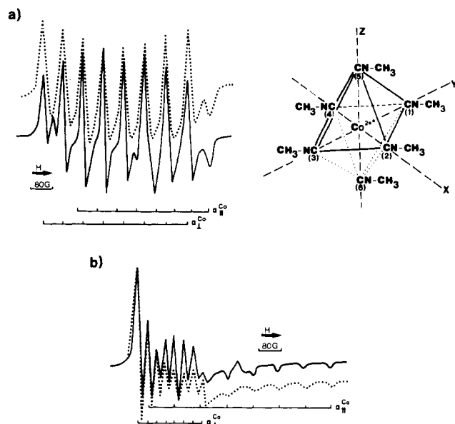
Figure 11. Intrazeolite cobalt(II)-methyl isocyanide complexes. (a) Experimental (—) and simulated (···) EPR spectra of [Co(CH 3 N 12 C) 6 ] 2+ . (b) Experimental (—) and simulated (···) EPR spectra of [Co(CH 3 N 12 C) 5 ] 2+ . Reprinted from ref 46; copyright 1975 Marcel Dekker.
