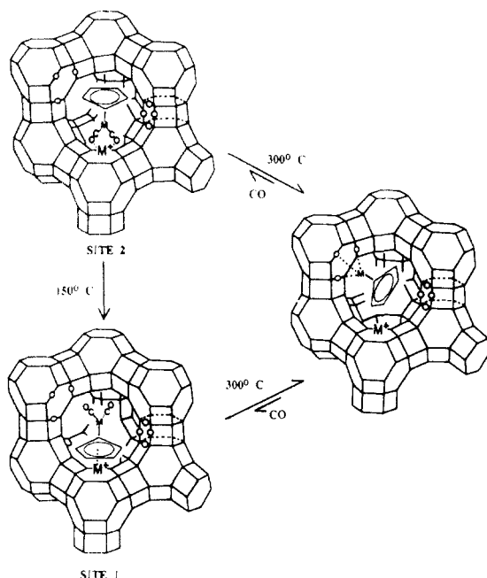
Figure 9. Effect of thermolysis on \text{CpM}(\text{CO})_2 in NaY. Apparent site interconversion occurs for M = \text{Ir} at 150^\circ\text{C} , while the half-sandwich, \text{CpIr} , is formed at higher temperatures. For M = \text{Rh} the half-sandwich is formed at lower temperatures. 36
