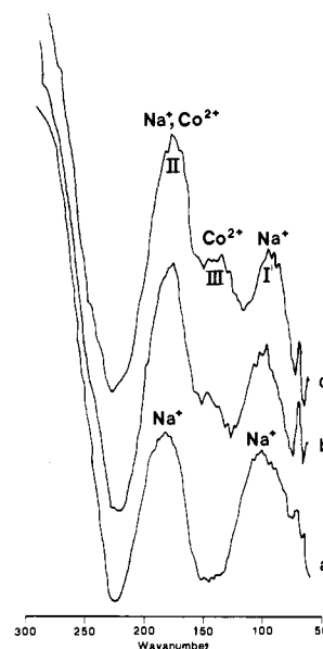
Figure 5. In situ FT-far-IR of (a) vacuum thermally dehydrated/deamminated \text{H}_{48}\text{Na}_9\text{Y} showing residual sodium sites and (b, c) the outcome of exposure to \text{Co}_2(\text{CO})_8 vapor for 5 and 15 min, respectively, showing the formation of \text{Co}^{2+} cations in accessible \alpha -cage sites II and III'. Reprinted from ref 27; copyright 1986 American Chemical Society.
