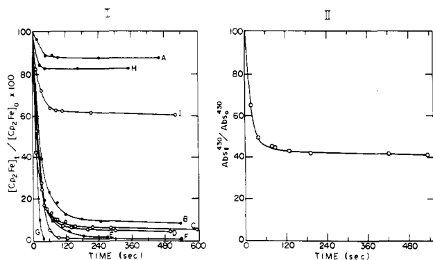
Figure 18. (I) Normalized absorbance plots of the impregnation rates of (A) \text{Cp}^*\text{Fe}/\text{Na}_{56}\text{Y} (D), (B) \text{Cp}_2\text{Fe}/\text{Na}_{56}\text{Y} , (C) \text{Cp}_2\text{Fe}/\text{H}_{16}\text{Y} , (D) \text{Cp}_2\text{Fe}/[\text{HPMe}_3]_8\text{Y} , (E) \text{Cp}_2\text{Fe}/\text{NaY} (D), (F) \text{Cp}_2\text{Fe}/\text{H}_8\text{Y} , (G) \text{Cp}^b\text{Fe}/\text{H}_{56}\text{Y} , (H) \text{Cp}_2\text{Fe}/\text{SiO}_2\text{-500} , and (I) \text{Cp}_2\text{Fe}/\text{Ca}_{28}\text{Y} (where \text{Na}_{56}\text{Y} (D) refers to a defect removed sodium Y zeolite that has been rigorously dehydrated/calced and \text{CH}_3\text{Li} treated). (II) Normalized absorbance plots of the impregnation rate of an equimolar mixture of \text{Cp}^*\text{Fe}/\text{Cp}_2\text{Fe}/\text{H}_{16}\text{Y} . Reprinted from ref 64; copyright 1989 American Chemical Society.
